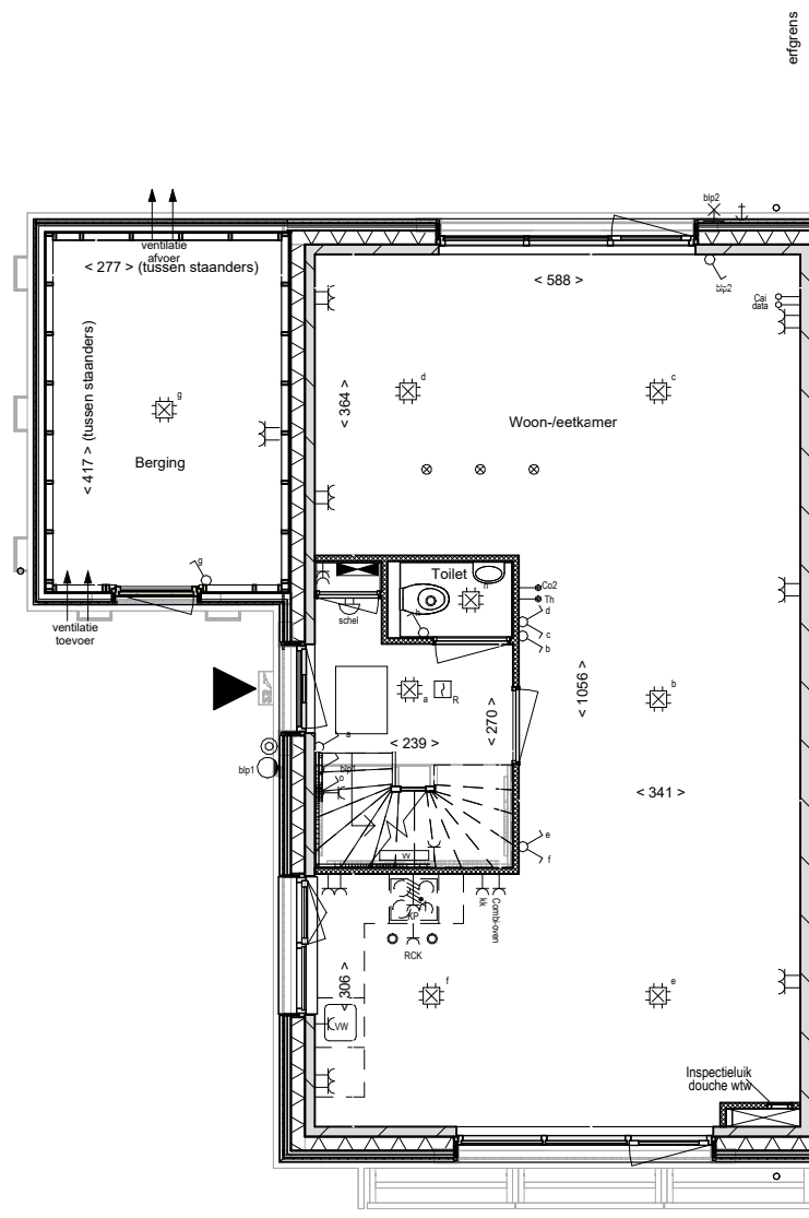
00 begane grond
