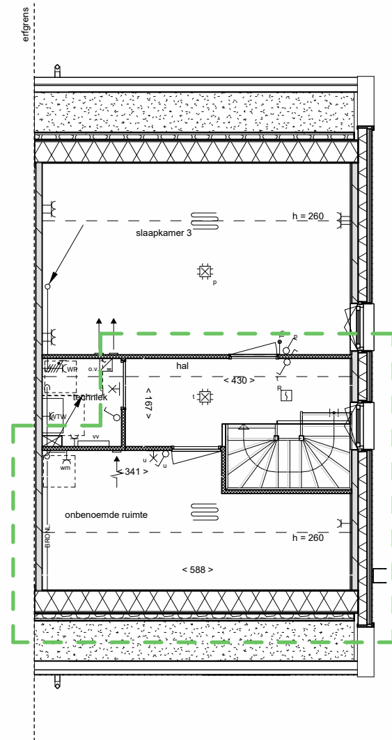
zolder
