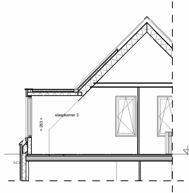
code 10500: dakkapel
